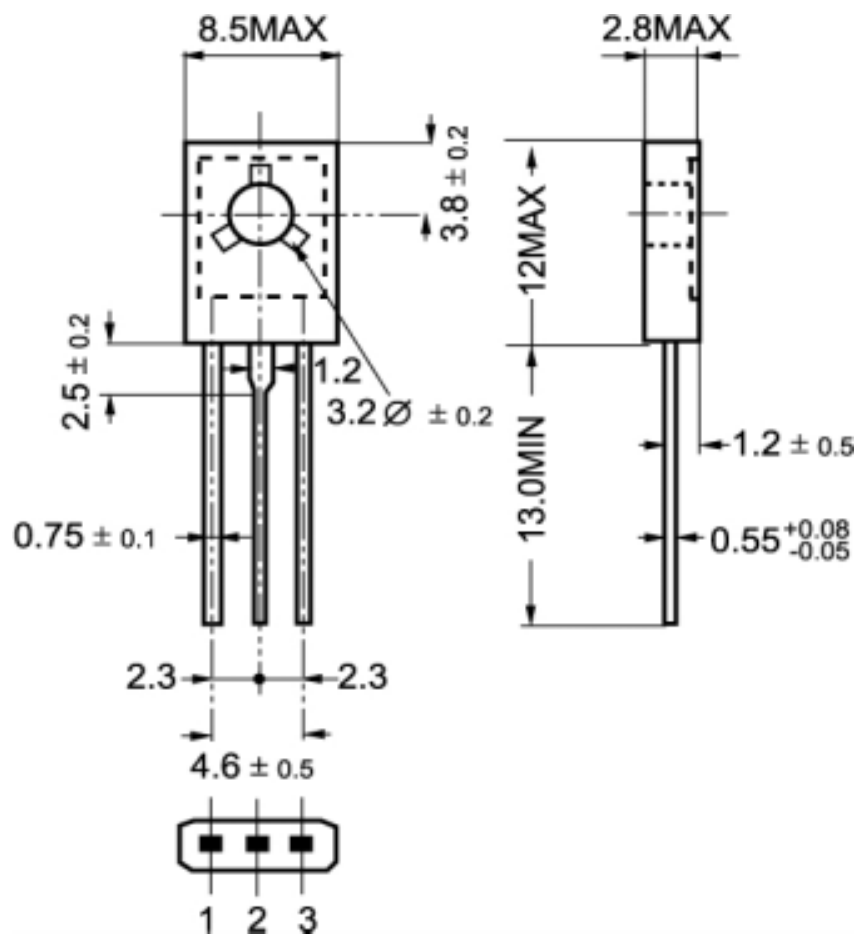
Fig.2 Outline dimensions
